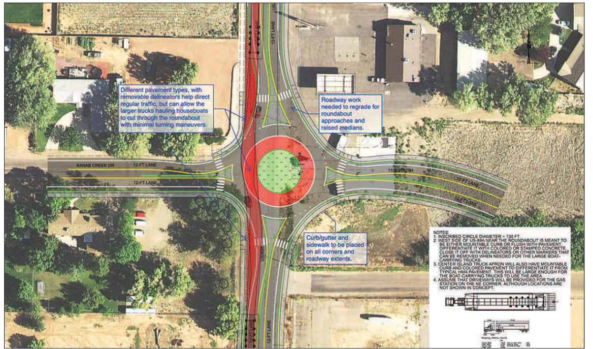
A preliminary consideration for how a roundabout might be installed on 89A via the Kanab City Council agenda packet.
